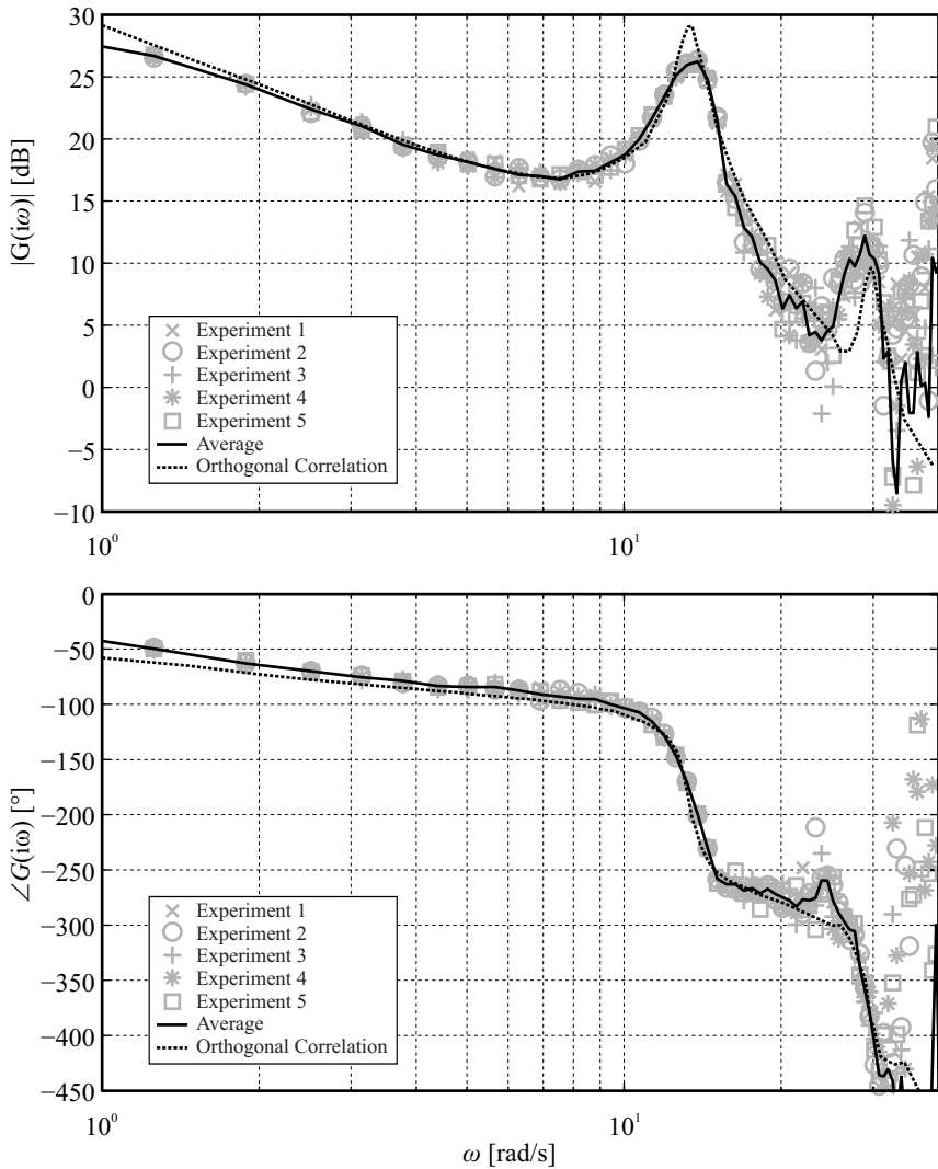
Fig. 4.11. Frequency responses determined from averaging multiple measurements with a rectangular pulse with noise \sigma = 1 . (solid line): Average of 5 frequency responses, (dashed line): Direct frequency response measurement with sinusoidal excitation and evaluation with orthogonal correlation (see Sect. 5.5.2)
