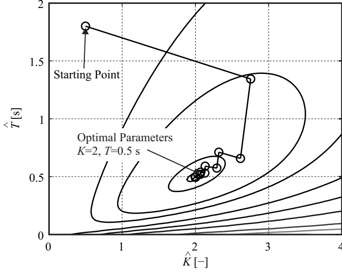
Fig. 19.5. Convergence of the steepest descent with contours of the cost function
