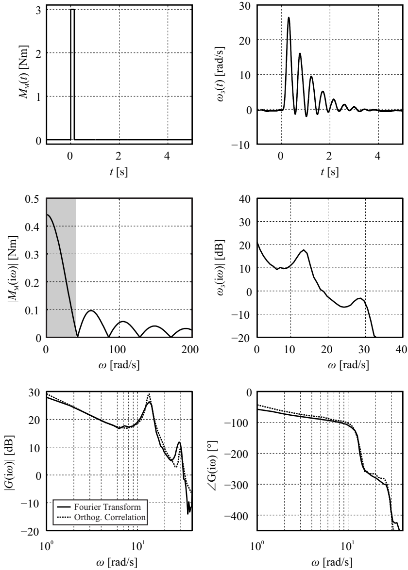
Fig. 4.9. Rectangular pulse response with step height u_0 = 3 \text{ Nm} and duration \Delta T = 0.15 \text{ s} and frequency response without noise
