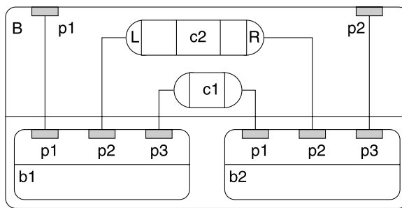
Figure 2.73. Structural hierarchy of SpecC example
