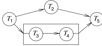
Figure 2.6. Hierarchical task graph
