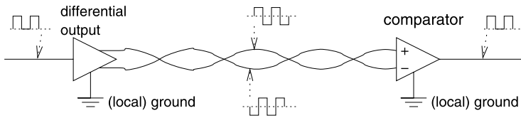
Figure 3.41. Differential signaling
