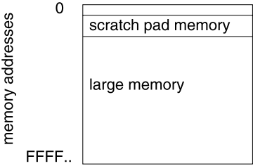
Figure 3.38. Memory map with scratch-pad included
