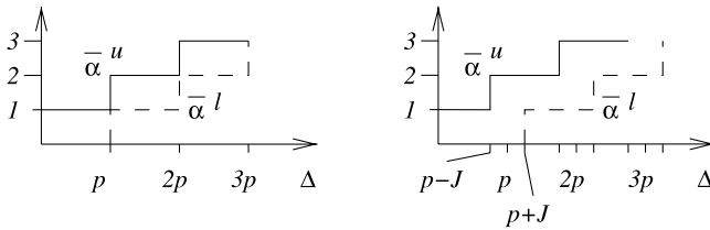
Figure 5.8. Arrival curves: periodic stream (left), periodic stream with jitter J (right)
