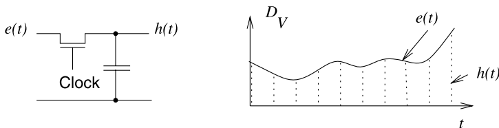
Figure 3.4. Sample-and-hold-circuit
