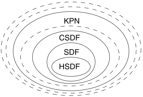
Figure 2.75. Expressiveness of data flow models
