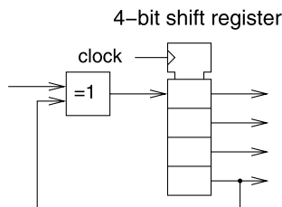
Figure 8.12. LFSR
