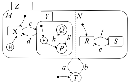
Figure 2.79. StateCharts example
