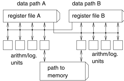
Figure 3.28. Partitioned register files for TMS 320C6xx
