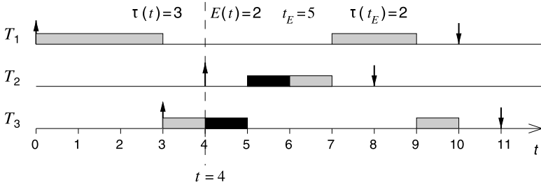
Figure 6.7. Schedule \tau
