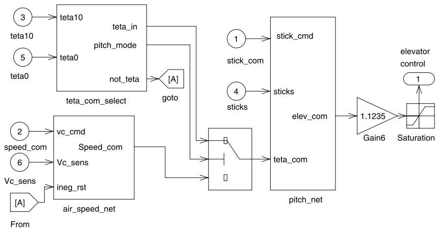
Figure 2.44. Simulink model
