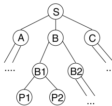
Figure 2.35. SDL hierarchy
