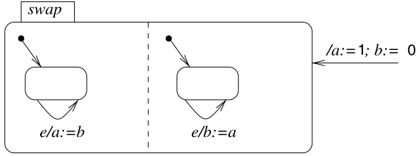
Figure 2.22. Mutually dependent assignments
