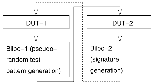
Figure 8.11. Cross-coupled BILBOs
